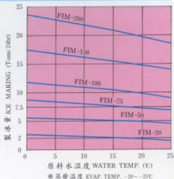
ICE MAKING CAPACITY CURVES
