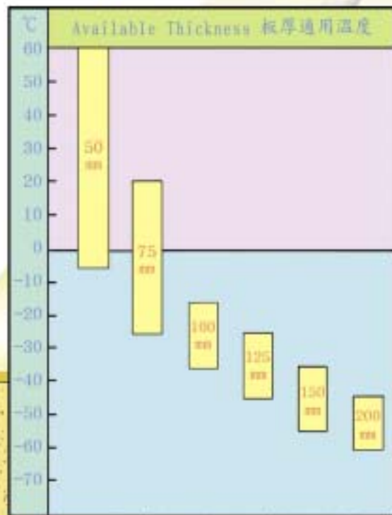
Thickness of Panel 庫板保溫厚度
