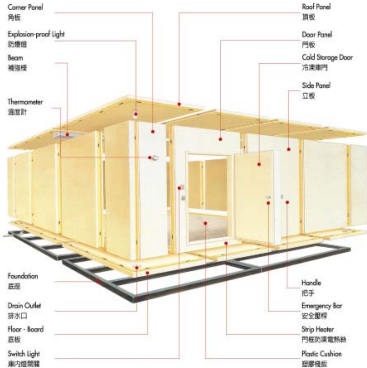
Example of Pre-fabricated Walk-in Cooler 組裝完成實例
